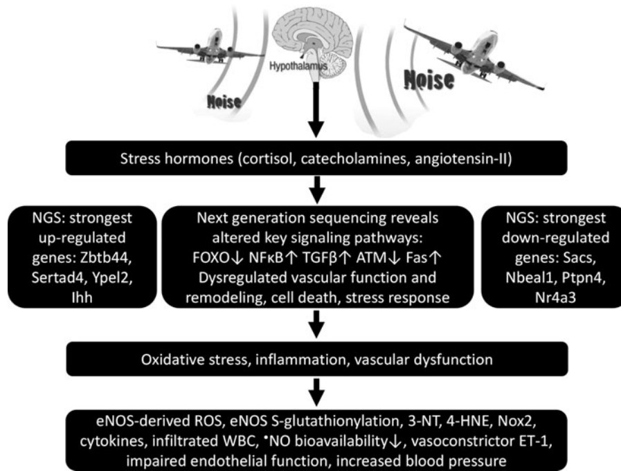
FIG. 16. Postulated mechanisms of noise-induced (cardio)vascular damage are based on the vascular functional and observational parameters as well as results from next-generation sequencing of our recent mouse study on the effects of aircraft noise exposure on the cardiovascular system. eNOS, endothelial nitric oxide synthase; Foxo, Forkhead-box-protein; Ihh, Indian hedgehog; *NO, nitric oxide; Nox2, NADPH oxidase isoform 2, ROS, reactive oxygen species, Ypel2, Yipee-like 2.
